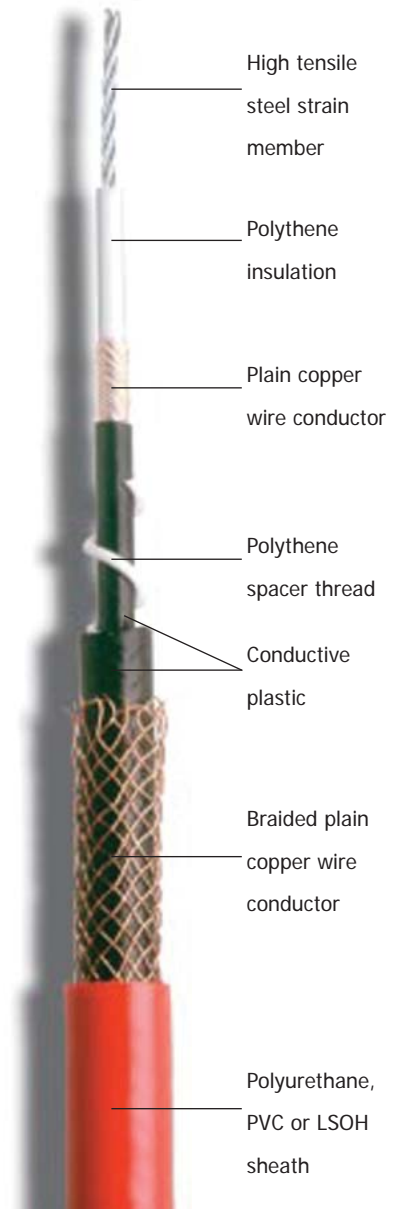
Pressline Cable
